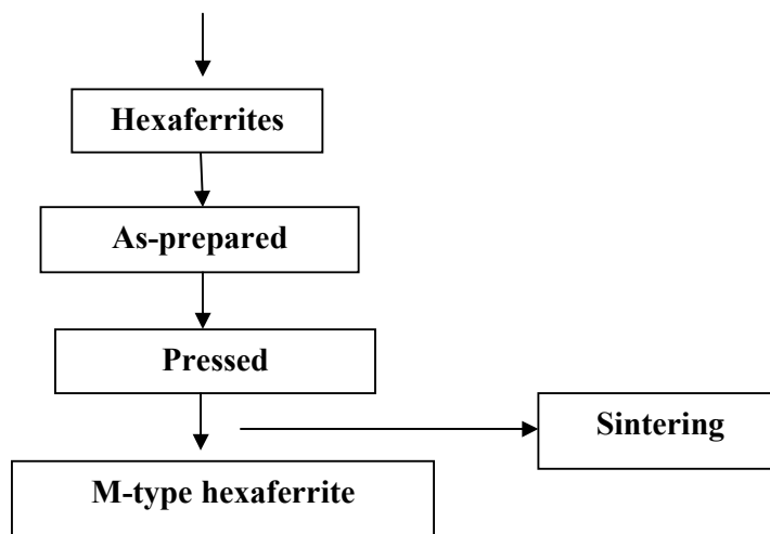
FIGURE 1. Flow-chart for synthesis of M-type hexaferrites Ba_{1-x}Al_xFe_{12}O_{19} nano powder by sol-gel auto-combination methods.
