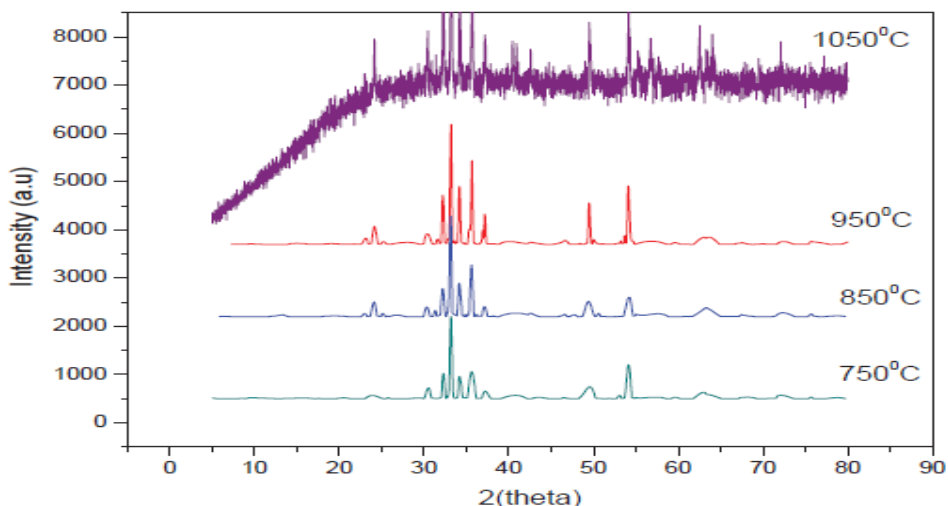
FIGURE 2. XRD patterns for Ba 1-x Al x Fe 12-y Mn y O 19 (x= 0.6 and y= 0.3) at different temperatures for 5h.
