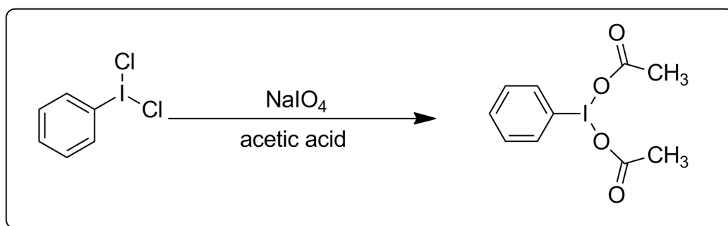
Scheme 1.3: Sodium periodate mediated synthesis method for DIB
