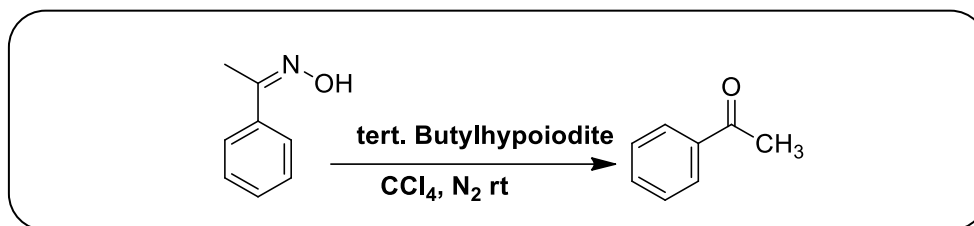
Scheme 1.30: Transformation of oximes to the corresponding carbonyl compounds using tert-butyl hypoiodite.
