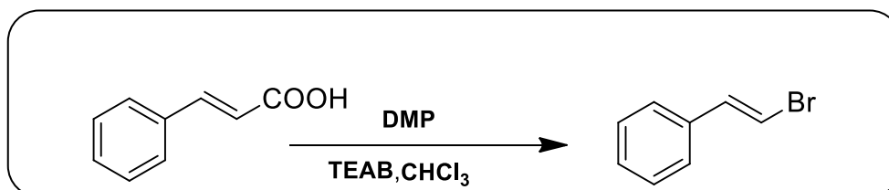
Scheme 1.29: Bromo-decarboxylation of cinnamic acid using DMP and TEAB.
