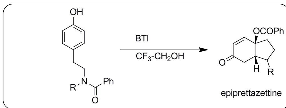
Scheme 1.14: Synthesis of epiprettazettine
