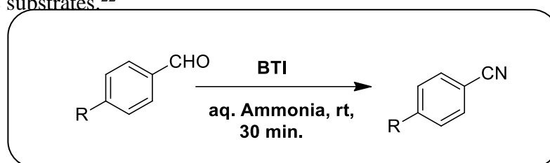
Scheme 1.21: Preparation of nitrile from aldehyde.
