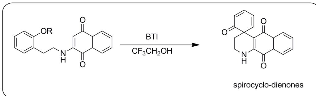
Scheme 1.18: Synthesis of spirocyclo-dienones
