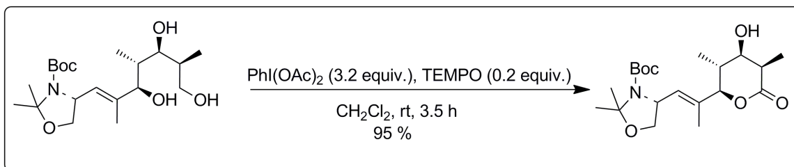
Scheme 1.11: Selective oxidation
