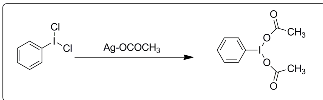
Scheme 1.4: Silver acetate mediated synthesis method for DIB
