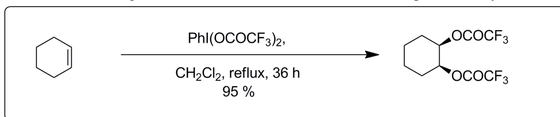
Scheme 1.13: Addition of Trifluoroacetate across C-C double bond
