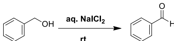
Scheme 1.25: Synthesis of aldehyde using aq \text{NaCl}_2 at rt.
