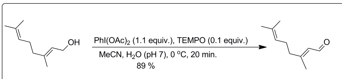
Scheme 1.10: Selective oxidation of -OH
