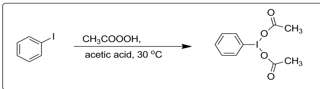
Scheme 1.2: Peracetic acid mediated synthesis method for DIB
