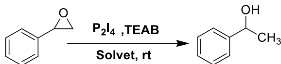
Scheme 1.23: Oxidative cleavage of styrene oxide to alcohol
