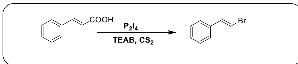
Scheme 1.28: Bromo-decarboxylation of cinnamic acid using DPTI and TEABr.
