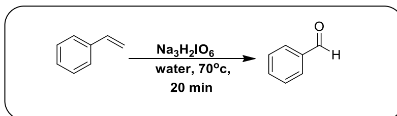
Scheme 1.22: Styrene to benzaldehyde using sodium paraperiodate.
