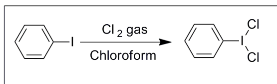
Scheme 1.1 Synthesis of (dichloriodo) benzene
