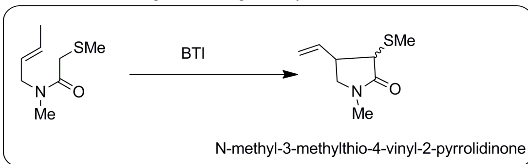
Scheme 1.17: Synthesis of substituted N-methyl,2-pyrrolidinone
