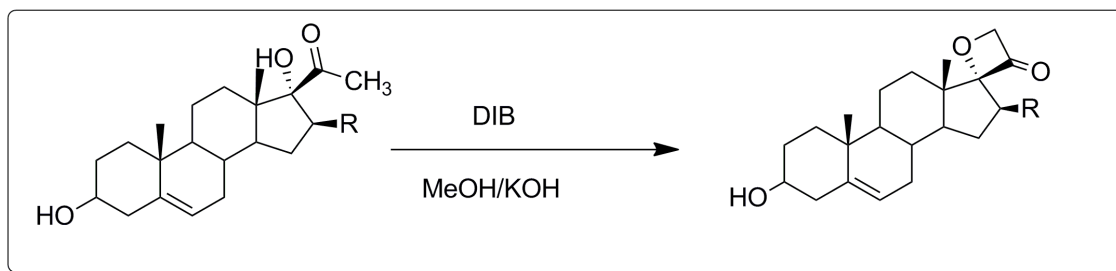
Scheme 1.12: Selective oxidation of C 17 -OH using DIB
