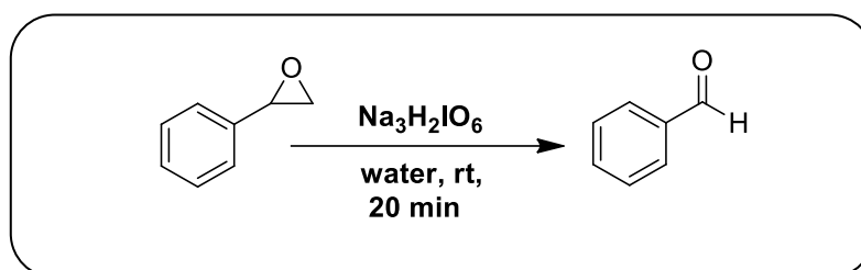
Scheme 1.20: Oxidative cleavage of styrene epoxide to benzaldehyde.
