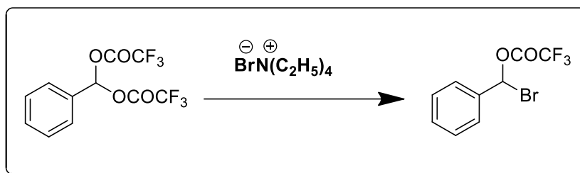
Scheme 1.19: BTI complex with TEAB
