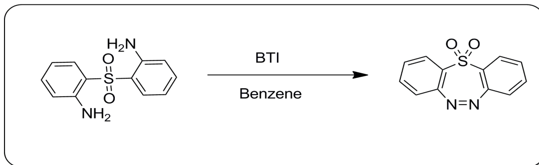
Scheme 1.15: Preparation of dibenzodiazepine
