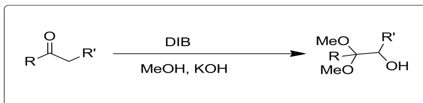
Scheme 1.5: DIB mediated oxidation of enolizable ketone
