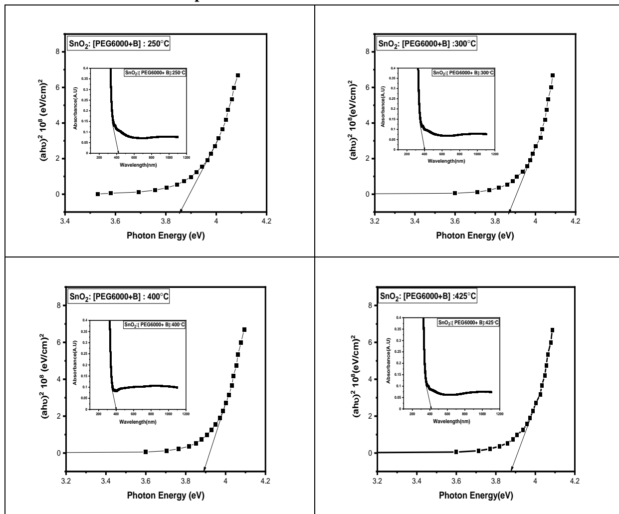
Figure 2: Optical absorbance and band gap of spray deposited SnO 2 : TX-100+B thin film at different substrate temperature
