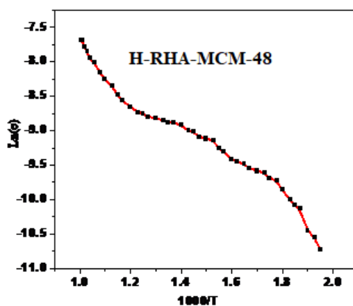
Fig. 2 : D.C. conductivity of RHA synthesized H-RHA-MCM-48 material.
