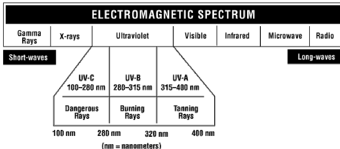
fig. 1. Electromagnetic spectrum showing UV A, UVB, UVC wavelength
