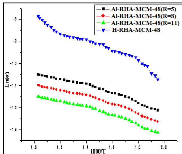
Fig. 4 : D.C. conductivity of fly ash synthesized H-RHA-MCM-48 and Al-RHA-MCM-48 (Si/Al=11, 9 and 5)
