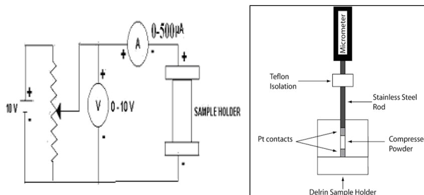
Fig. 1 : Circuit diagram and Sample Holder to measure DC conductivity of a given sample
