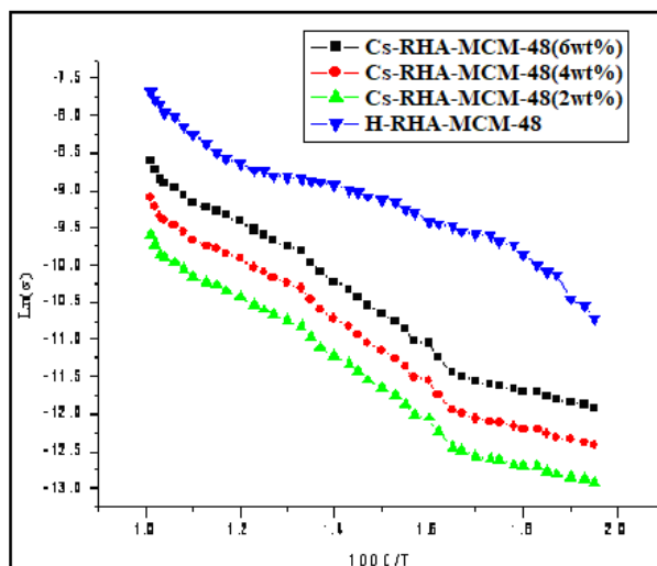
Fig. 3 : D.C. conductivity of fly ash synthesized H-RHA-MCM-48 and Cs-RHA-MCM-48 (2wt %, 4wt % and 6 wt %)
