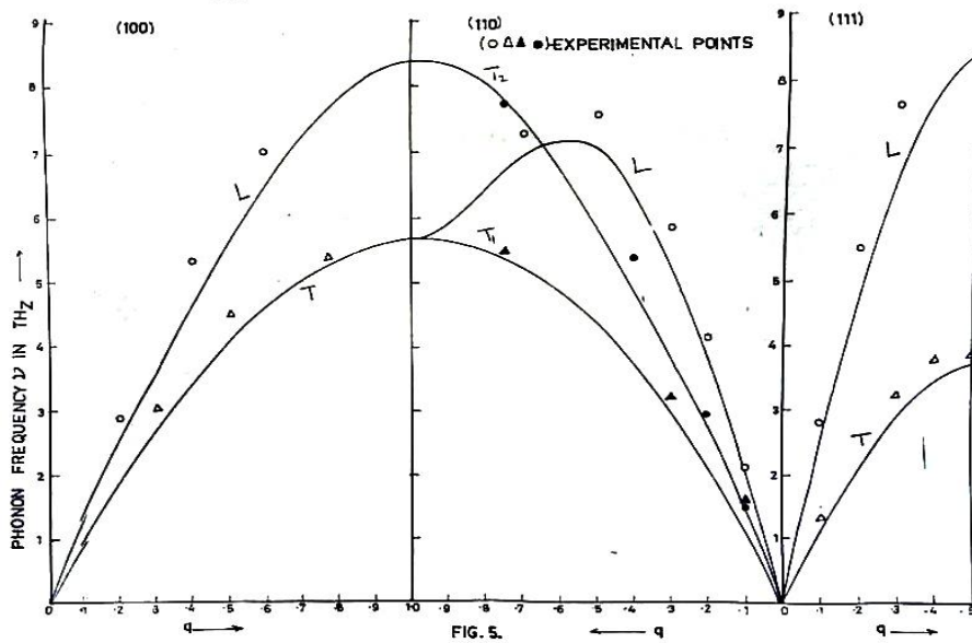
[PHONON DISPERSION CURVE FOR THORIUM]
