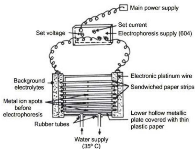
The Electrophoresis cell showing the sandwiched paper strips and the water supply.
