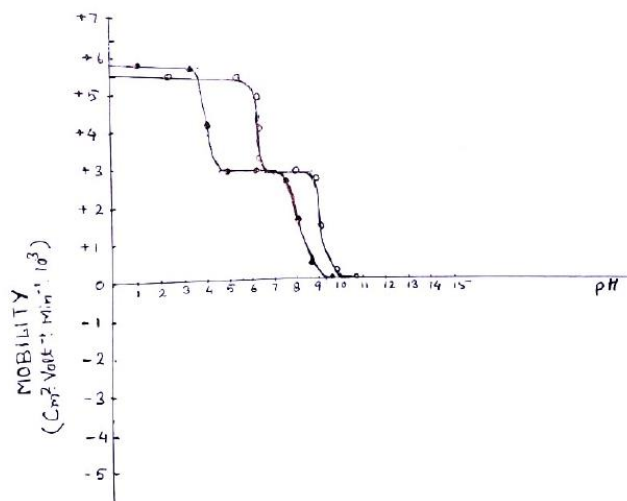
Mobility Curves
