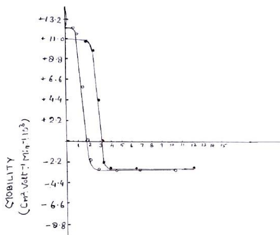
Fig.3- Mobility curve for the Metal-NTA system. [O] Cu (II)-NTA and (●) Co (II) – NTA. Concentration of NTA = 0.001M, Concentration of Cu (II) and Co (II) = 0.005M, ionic strength = 0.1M : temperature = 35°C. The paper strips were spotted with 0.1 \mu l of sample solution and glucose (for making electro-osmotic correction)
